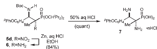
Scheme 1 Conversion of \alpha -nitrophosphonates to \alpha -amino phosphonates and \alpha -amino phosphonic acids.
